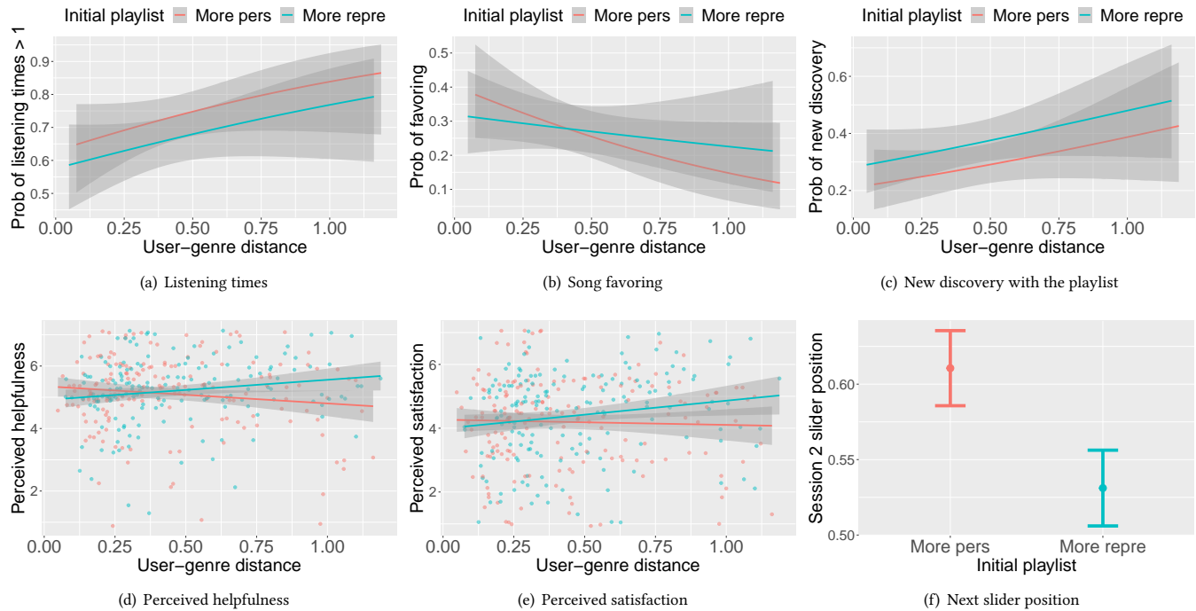
Figure 3: Reported listening behavior and experience after Session 1. In (d) and (e), the scatter plot shows the original distribution (jittered), with the shaded area indicating 95% confidence interval.
