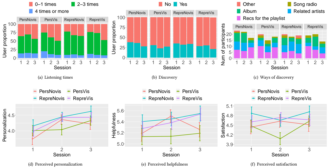
Figure 5: Reported listening behavior and user experience over sessions. In (d) to (f), the error bar indicates the standard error.
